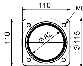
5-Flange
